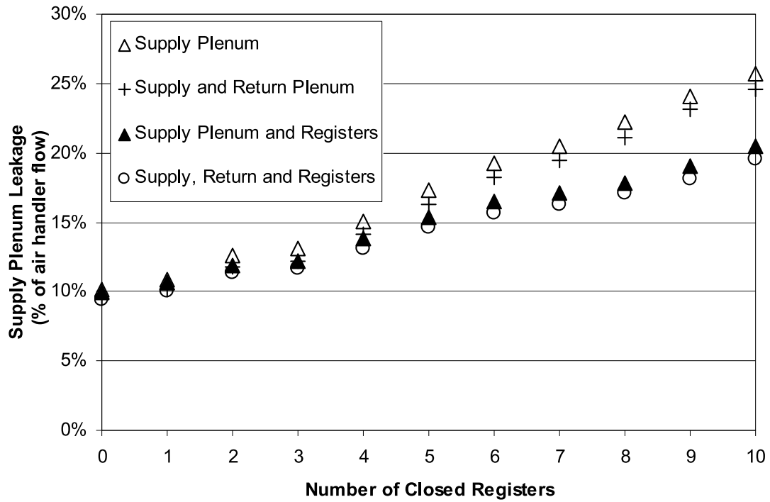
Figure D21. Supply plenum leakage as a fraction of air handler flow - Near registers closed first
