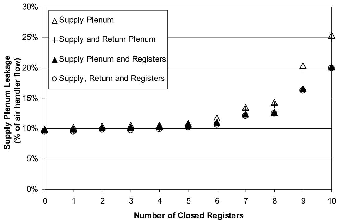
Figure D22. Supply plenum leakage as a fraction of air handler flow - Far registers closed first
