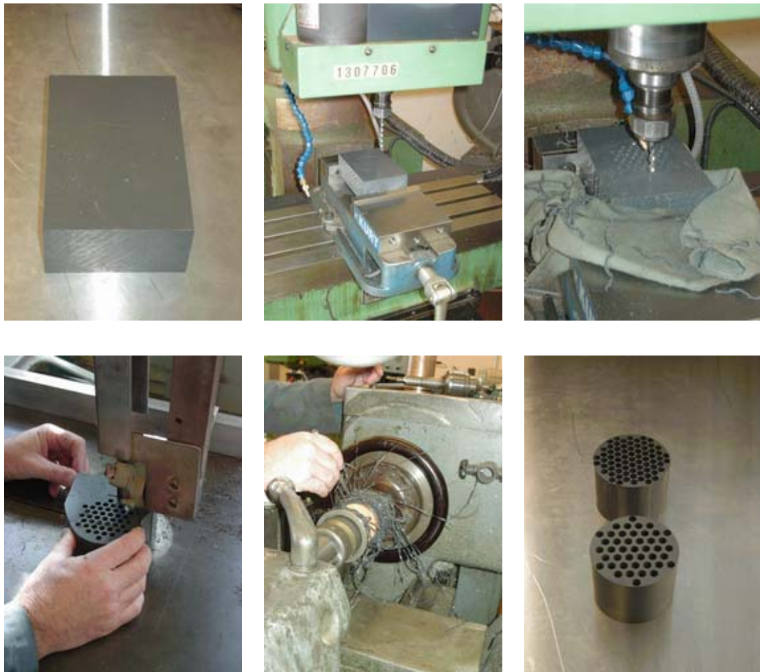
Figure A4. Construction of controlled pressure exponent boot leaks machined from solid PVC blocks.
