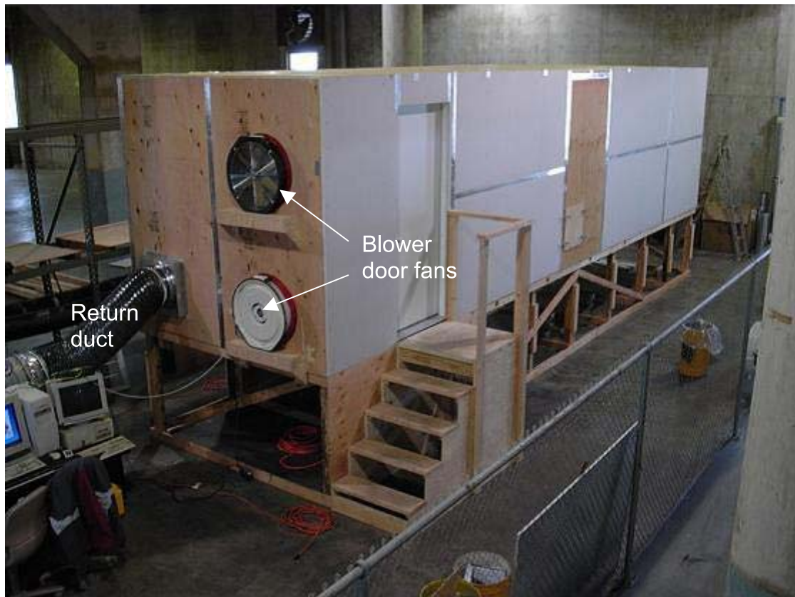
Figure 1. Completed test chamber inside warehouse showing the return duct connection and blower door fans (before supply duct installation).
