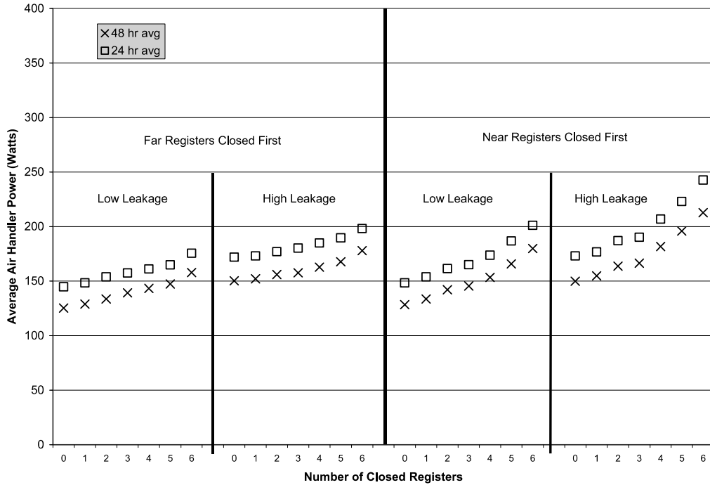
Average Air Handler Power (Watts) - Climate Zone 3
