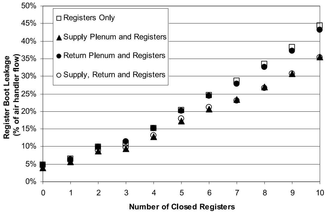
Figure D25. Register boot only leakage as a fraction of air handler flow - Near registers closed first
