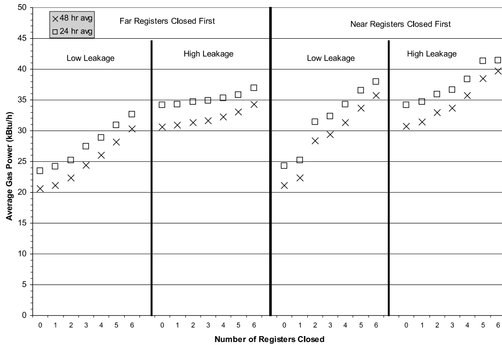
Average Gas Power - Climate Zone 12
