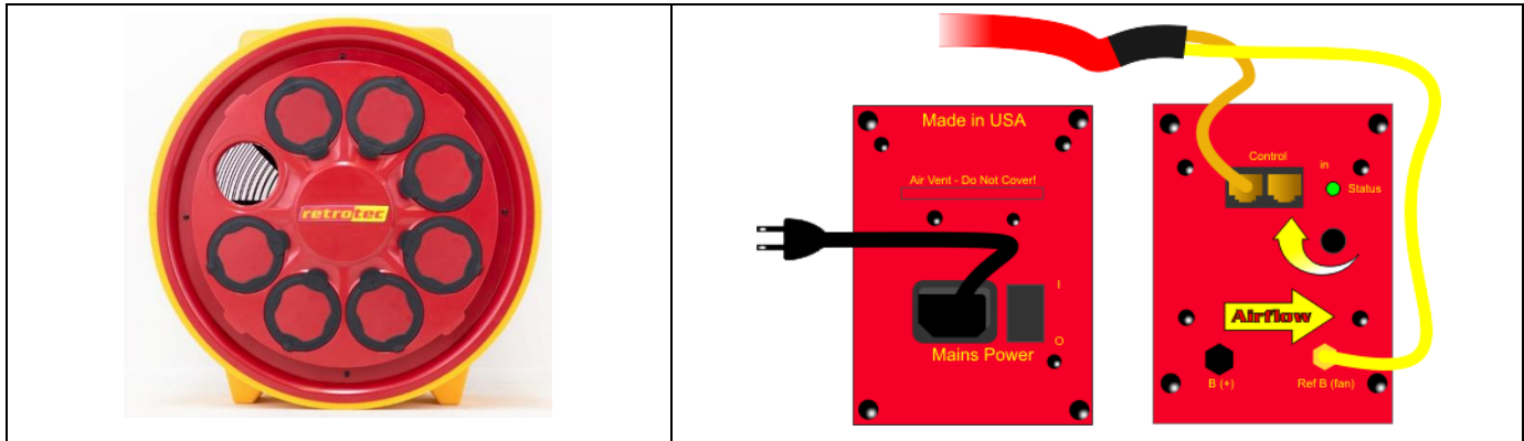
Figure 6: Model 5000 fan with two electrical plates containing power connection and switch, dual Control Ports and manual speed knob.
