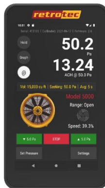
DM32X digital gauge has been turned on and is ready for action.
