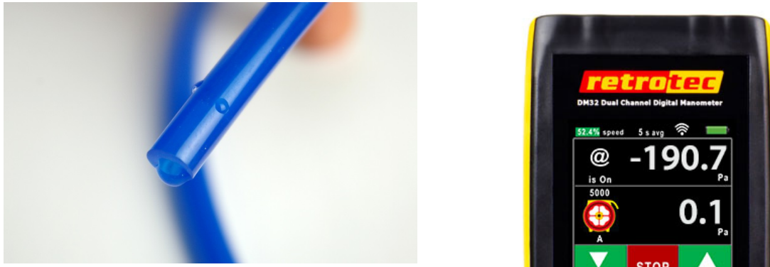
Figure 68: Water in the reference tube (left); high fixed pressure due to water (right).
